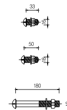
⊕ Bolt
