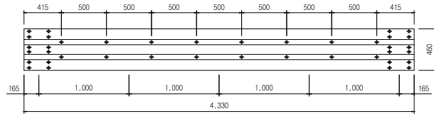
⊕ Detailed drawing of "A - A" (3.2*460*4,330)
