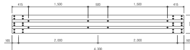
⊕ Detailed drawing of "B - B" (3.2*460*4,330)
