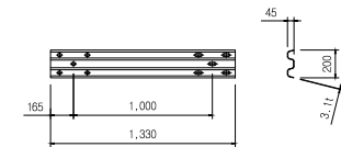
⊕ YC Rail SCALE: NONE
