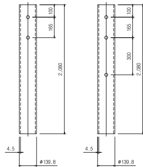
⊕ Post (4.5*139.8*2080)
