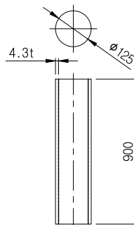
③ Post Reinforcement Structure SCALE: NONE
