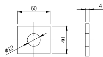
④ Square washer SCALE: NONE
