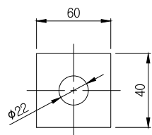
④ Square washer SCALE: NONE
