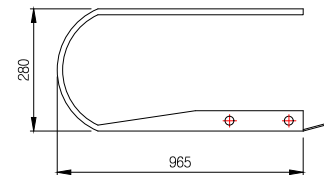
⑧ Round Rail SCALE: NONE
