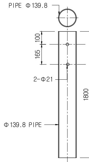
ROUND RAIL SCALE : NONE
