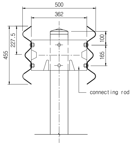
Cushion bracket assembly drawing SCALE : NONE
