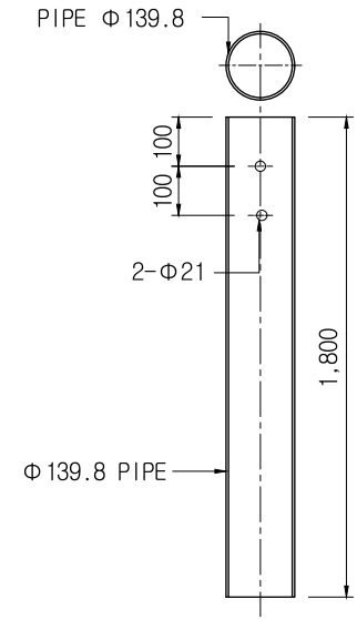
PIPE POST SCALE : NONE
