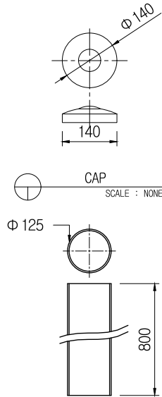
Post Reinforcement Structure SCALE : NONE
