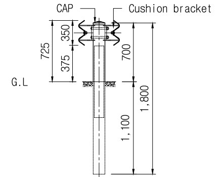
SIDE ELEVATION SCALE : NONE
