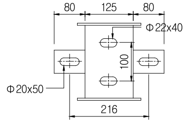
Front view SCALE : NONE
