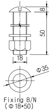
Bolt SCALE : NONE
