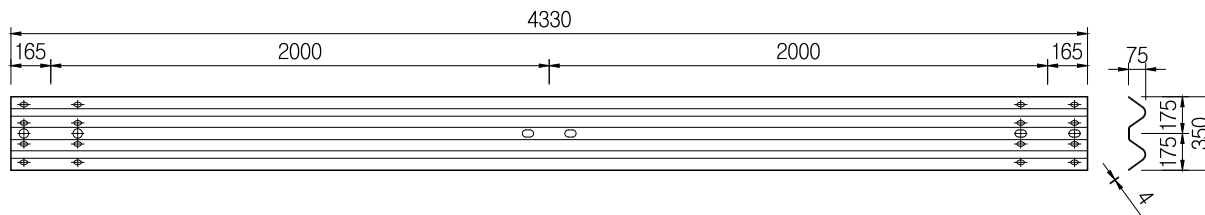
Guard Rail SCALE : NONE
