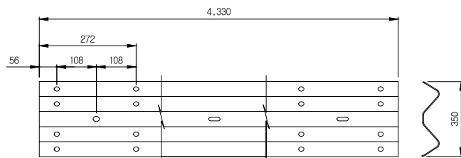
Standard rail SCALE: NONE
